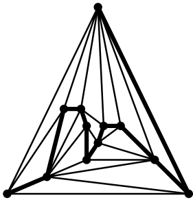
Figure 4: Every 4-connected planar graph has stack number at most 2 (since it is Hamiltonian)
