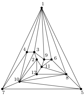
Figure 5: A 3-queue layout of a given planar graph.
