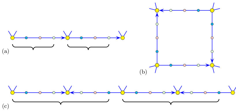
Figure 7: Illustration for Lemma 9.12.
