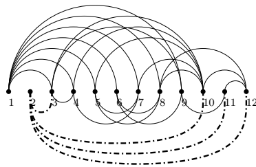
Figure 5: A 3-queue layout of a given planar graph.
