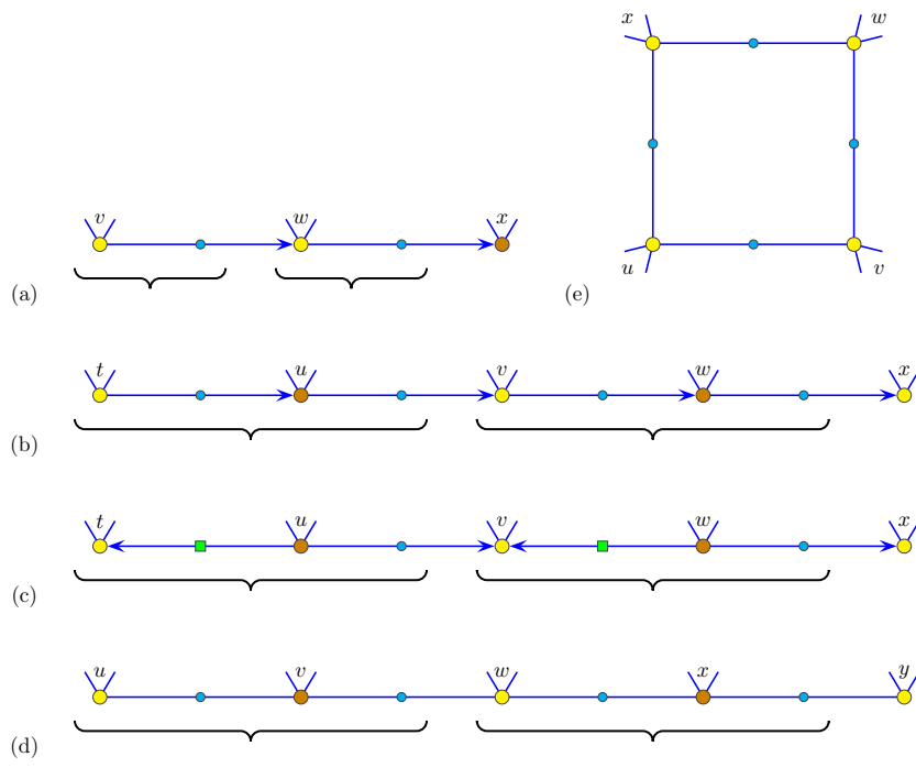
Figure 6: Illustration for Lemma 9.6.
