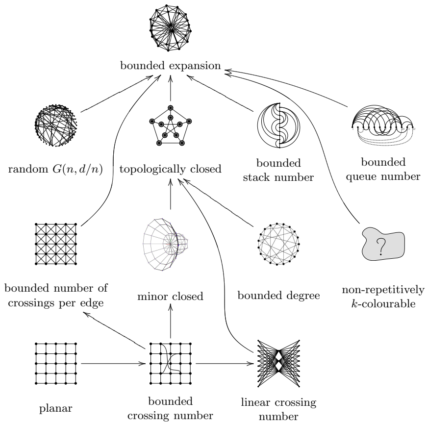
Figure 1: Classes with Bounded Expansion. The results about classes with bounded crossings, bounded queue-number, bounded stack-number, and bounded non-repetitive chromatic number are proved in this paper.
