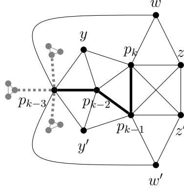
Figure 4: Vertices w and w' and position of T .
