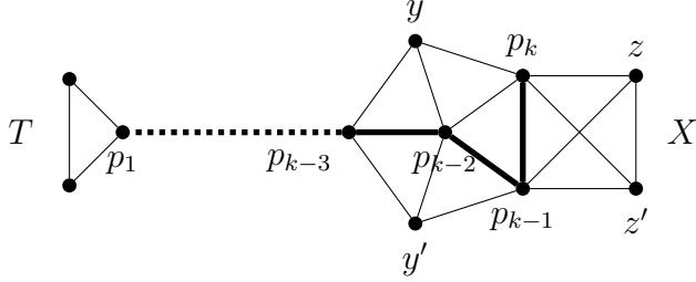
Figure 3: Positions of T , X , y and y' .
