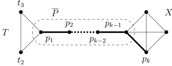
Figure 2: Paths P and \overline{P} connecting dangerous configurations.
