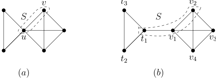
Figure 1: The configurations of Claims 11 and 12.
